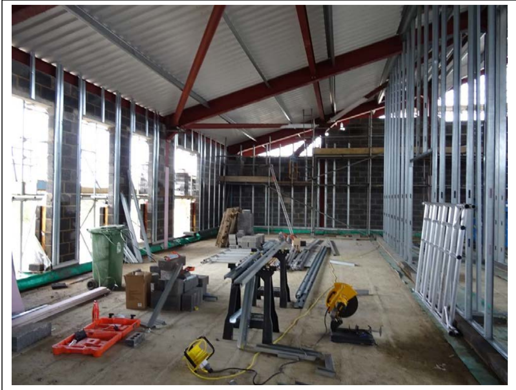
Blockwork is continuing, internal walls are underway
