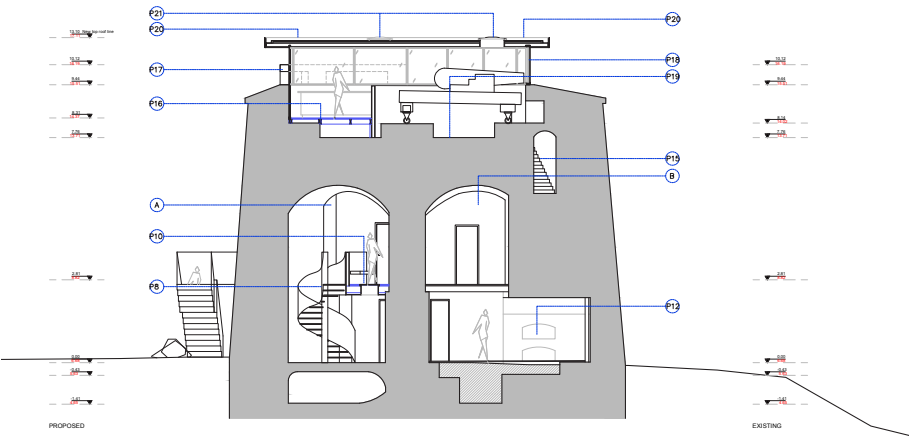
Proposed Martello Tower 64 proposed section AA
