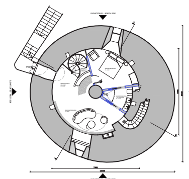
MARTELLO 64 PROPOSED FIRST FLOOR KEY PLAN / Scale 1:1250 @A3
