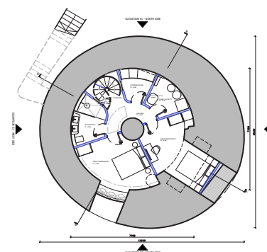
MARTELLO 64 PROPOSED GROUND FLOOR KEY PLAN / Scale 1:1250 @A3
